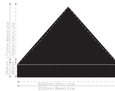
Right Canopy Panel
