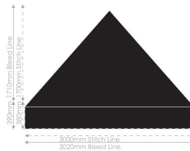
Front Canopy Panel
