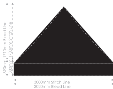
Left Canopy Panel
