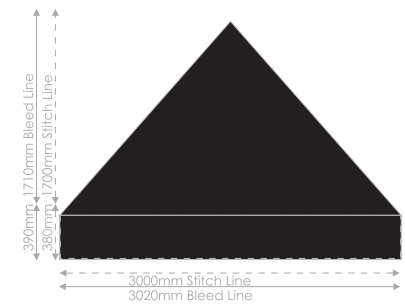
Back Canopy Panel
